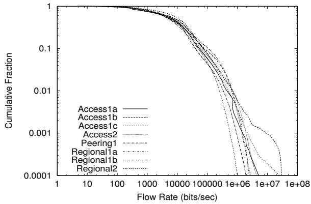
Figure 1: Complementary distribution of flow rates
