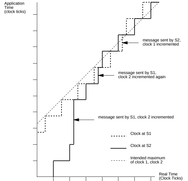
Figure 3: Clock synchronisation failure due to clock granularity being greater than transmission delay
