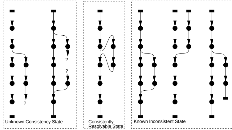
Figure 9: Known consistency, unknown state, and known inconsistency
