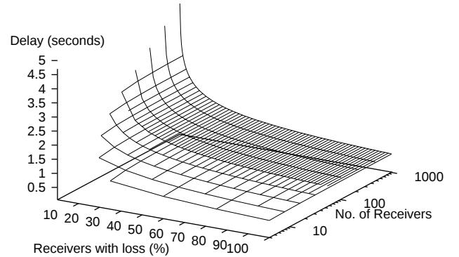
Figure 5: Expected delay before a retransmission request (RTT=250ms)
