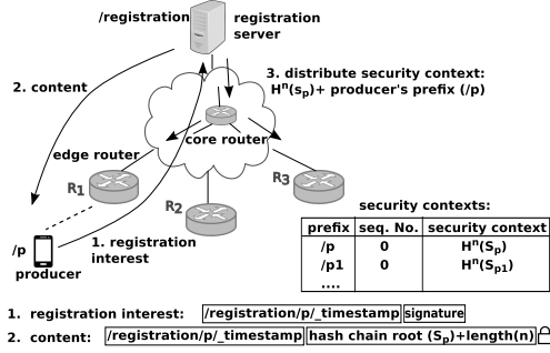
Figure 3: Bootstrap phase
