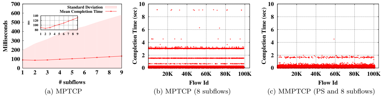
Figure 1: Short flow completion times in a simulated 4:1 over-subscribed FatTree topology consisting of 512 servers. One third of the servers run long (background) flows. The rest run short flows (70KBs each) which are scheduled according to a Poisson process). All flows are scheduled based on a permutation traffic matrix.
