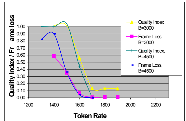
Figure 8. QBone Streaming ( Lost clip/1.5 Mbps encoding): Video Quality & Frame Loss vs Token Rate.
