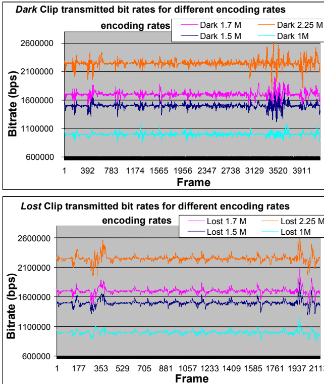
Figure 6. Instantaneous Transmission Rates of MPEG-1 Clips for Different Encoding Rates.
