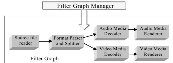
Figure 1. Directshow TM filter graph and graph manager.
