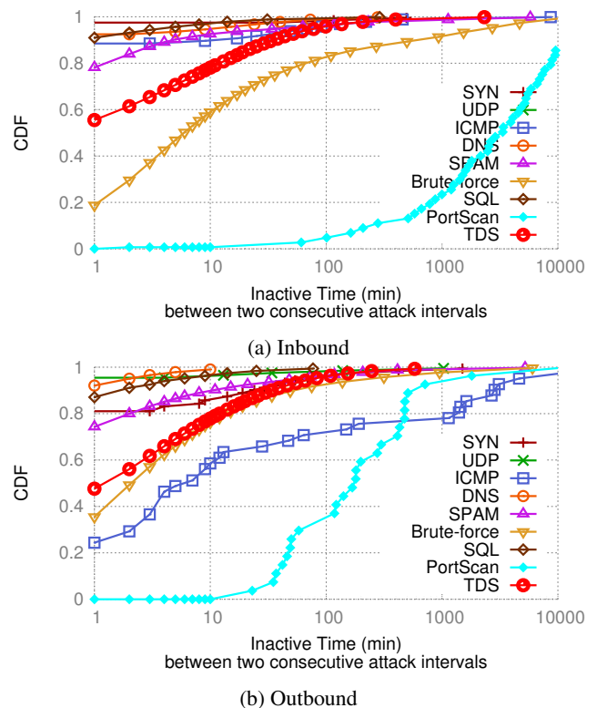
Figure 1: The distribution of inactive time for each attack type; the x-axis is on log-scale.
