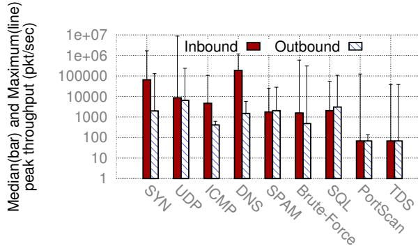
Figure 8: Median and maximum attack throughput across VIPs; the y-axis is on log-scale.
