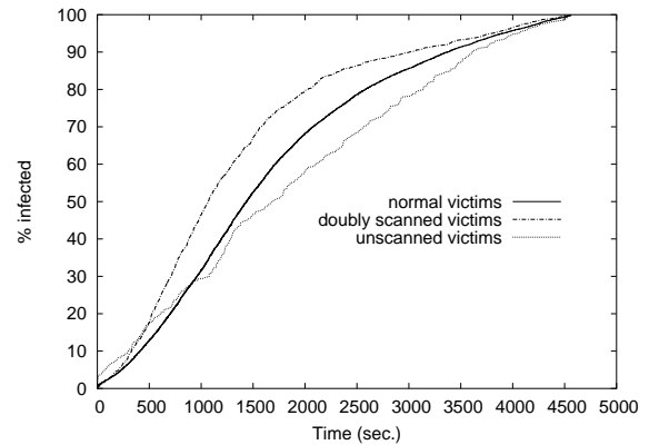
Figure 3: Growth curves for victims whose addresses were scanned once per orbit, twice per orbit, or not at all.
