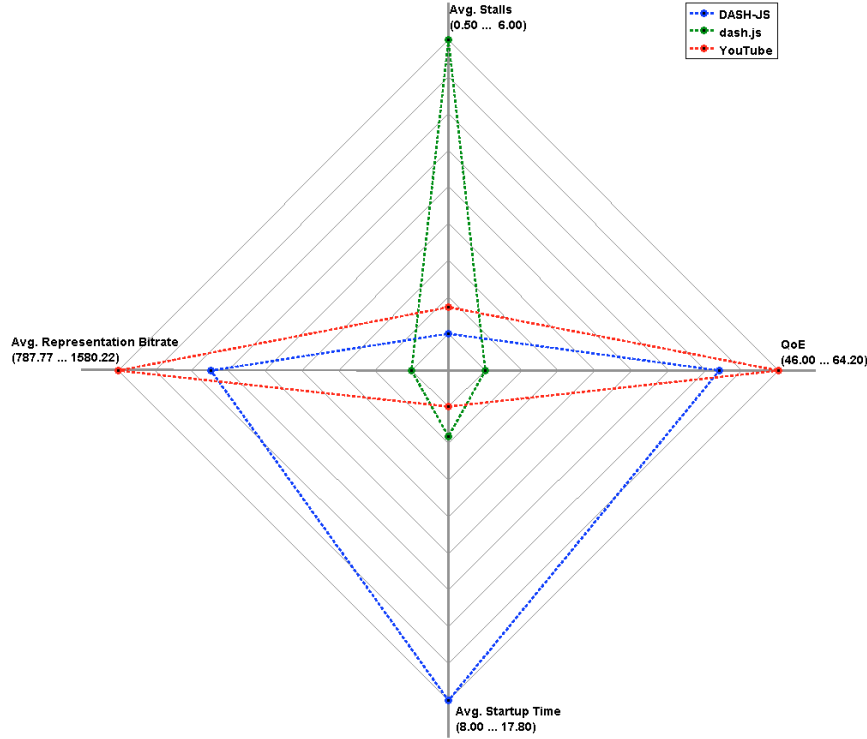
Figure 3: Overview of the results for the evaluated DASH-enabled Web clients.
