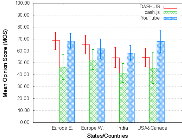
Figure 4: MOS grouped by the regions and presented for each Web client.
