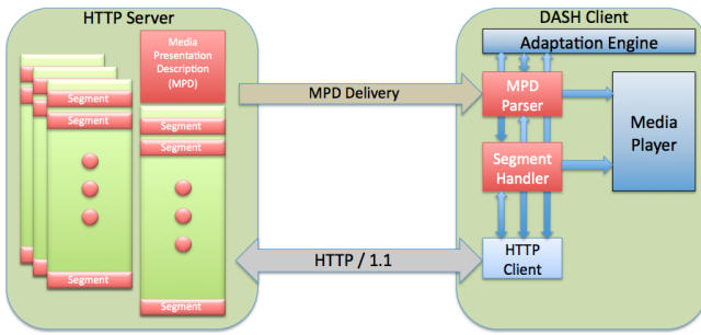
Figure 1: MPEG-DASH-based System Architecture.
