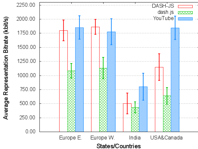
Figure 5: Average representation bitrate selected by each client grouped by region.
