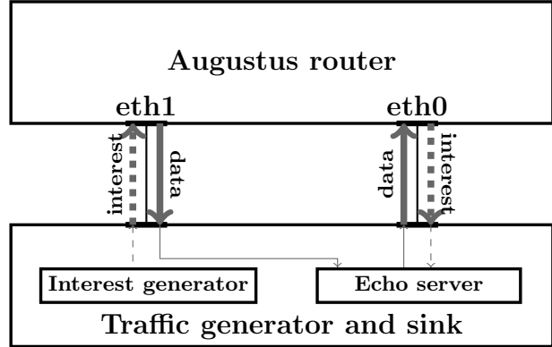
Figure 4: Traffic flow for the router evaluation experiments.
